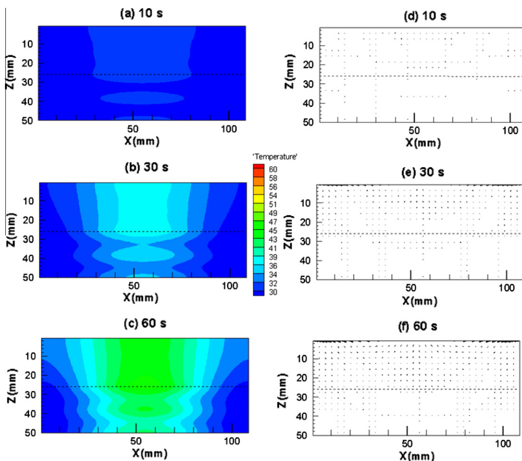
Fig. 10. Contours of temperature ( ^{\circ}\text{C} ) in the porous packed bed (a)–(c) and velocity vectors of water in porous materials, (d)–(f) at 10, 30, 60 s. Alumina balls are on top and Glass beads are in the bottom, both layers have diameter and porosity equal to 0.15 mm and 0.385, respectively.
