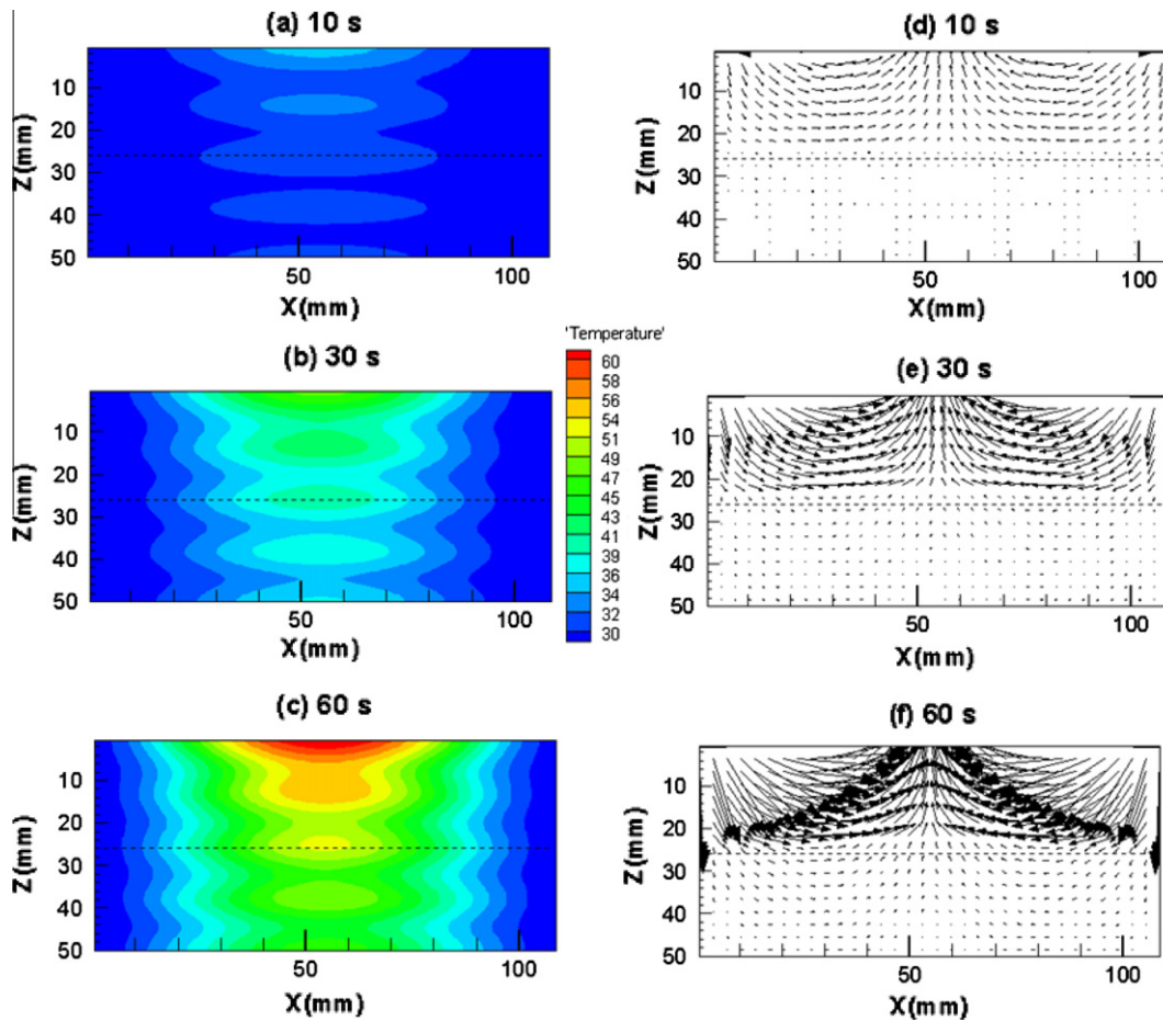
Fig. 7. Contours of temperature (°C) in the porous packed bed (a)–(c) and velocity vectors of water in porous materials, (d)–(f) at 10, 30, 60 s. Glass beads with diameter of 0.4 mm and 0.15 mm on the top and bottom layers, respectively. Both layers have a porosity of 0.385.
