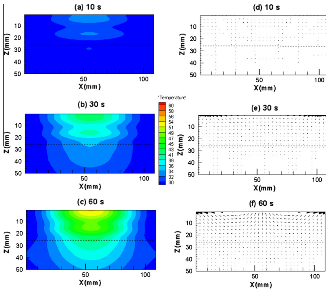
Fig. 9. Contours of temperature (°C) in the porous packed bed (a)(c) and velocity vectors of water in porous materials, (d)(f) at 10, 30, 60 s. Glass beads are on top and alumina balls are in the bottom, both layers have diameter and porosity equal to 0.15 mm and 0.385, respectively.
